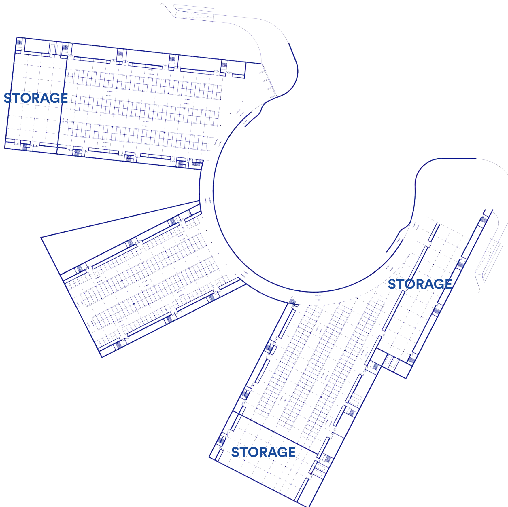
PARKING BASEMENT 1 1/1500
