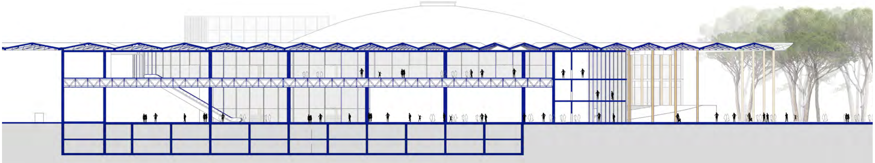
HALL II LONGITUDINAL SECTION (B) 1/500
