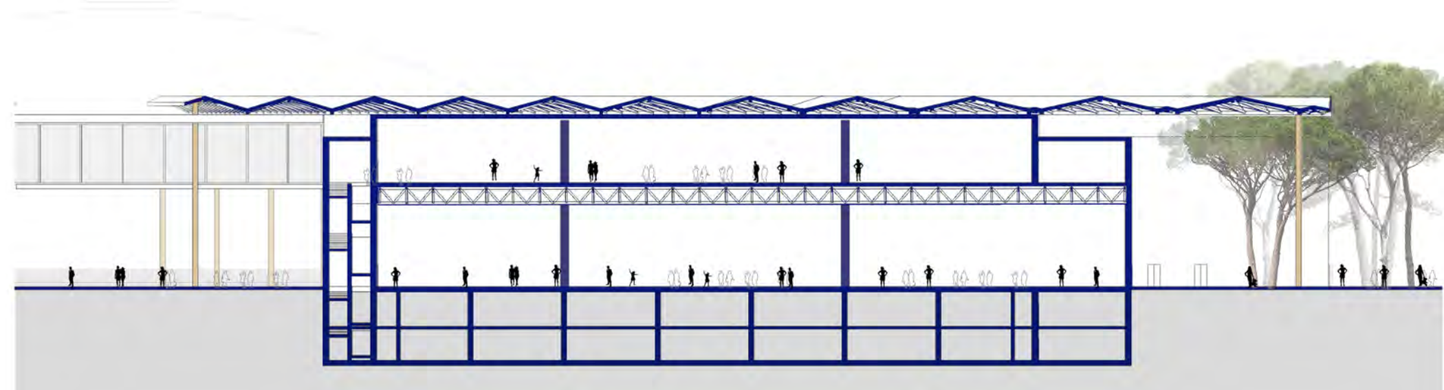
HALL II CROSS SECTION (A) 1/500
