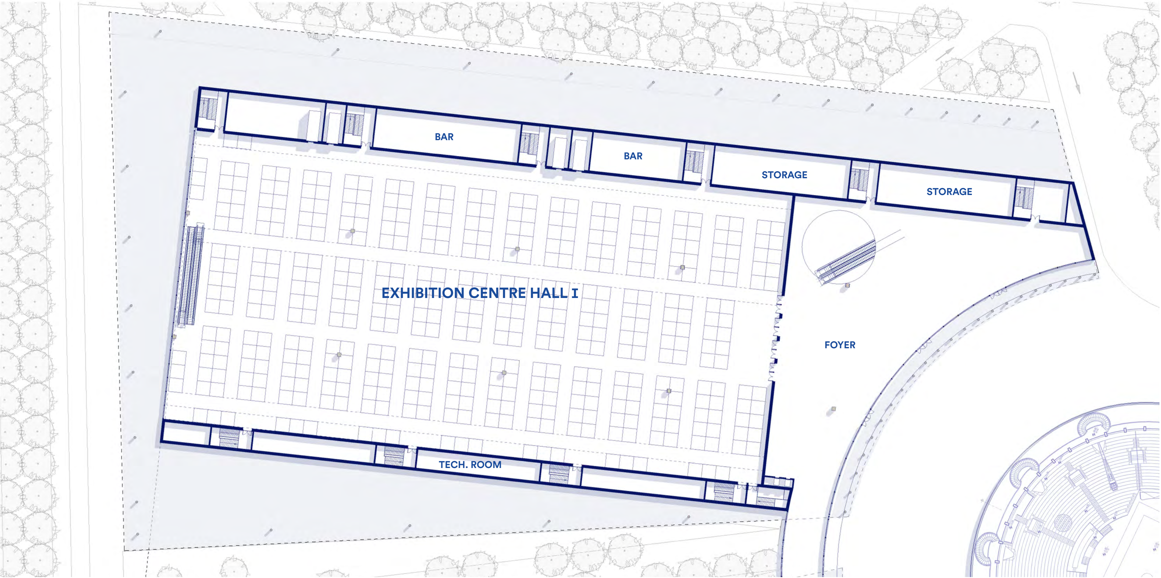
HALL I FIRST FLOOR 1/500
