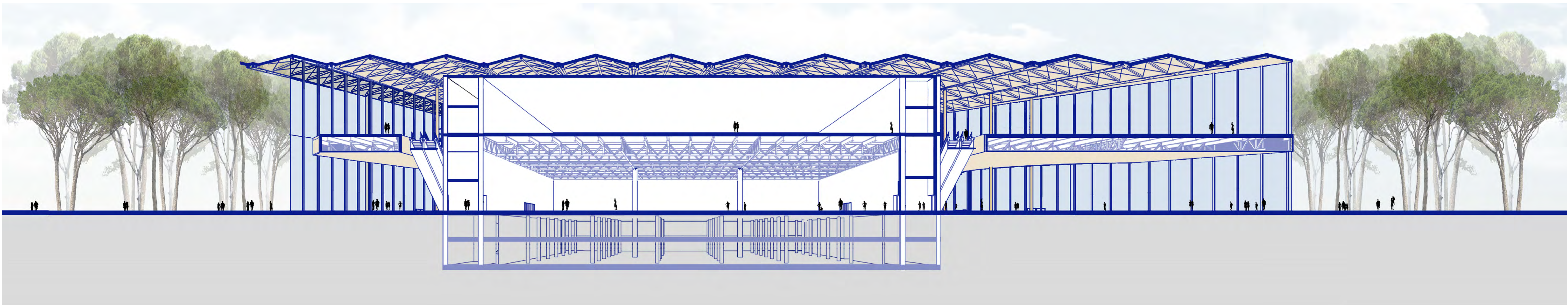
CONGRESS CENTER CROSS SECTION 1/250
