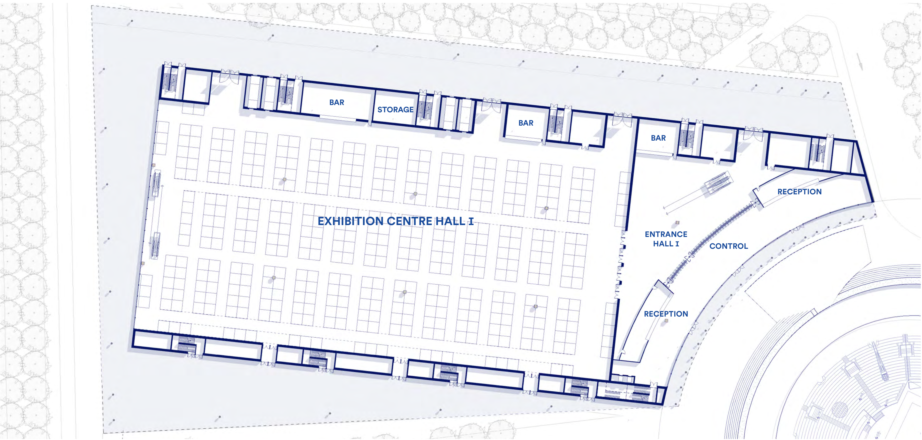
HALL I GROUND FLOOR 1/500
