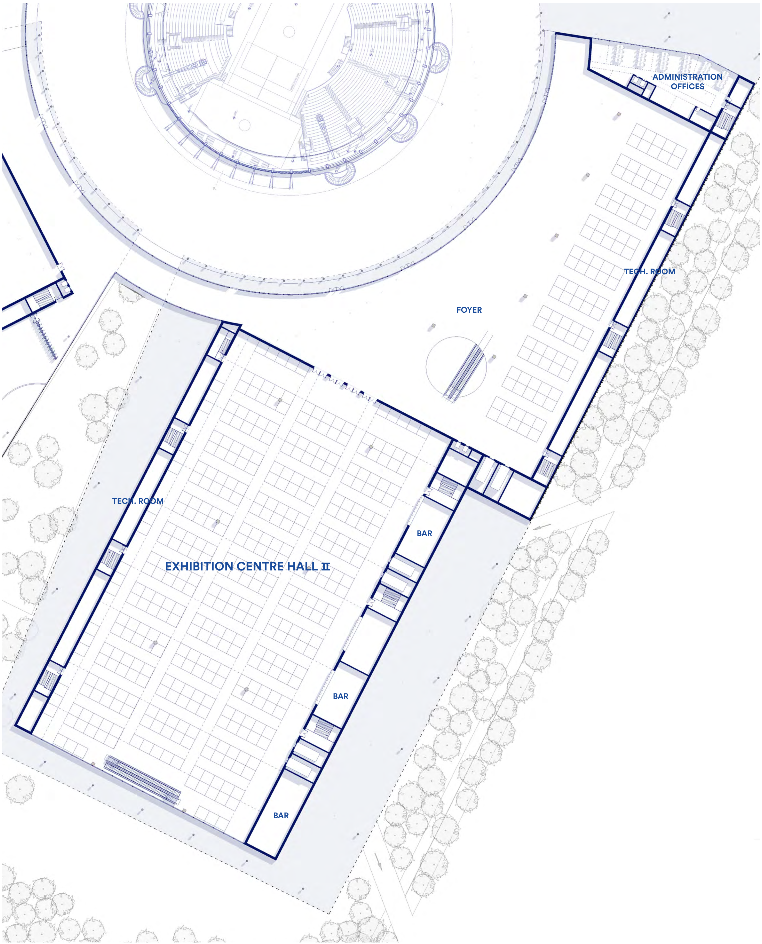
HALL II FIRST FLOOR 1/250
